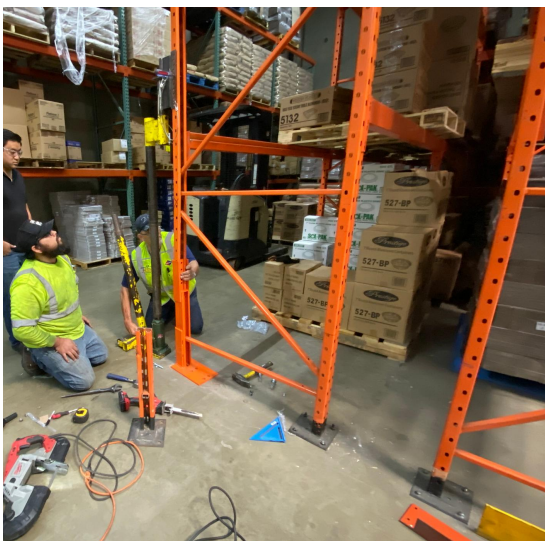
STEP #3 - REPLACE DAMAGED RACKING WITH KIT
