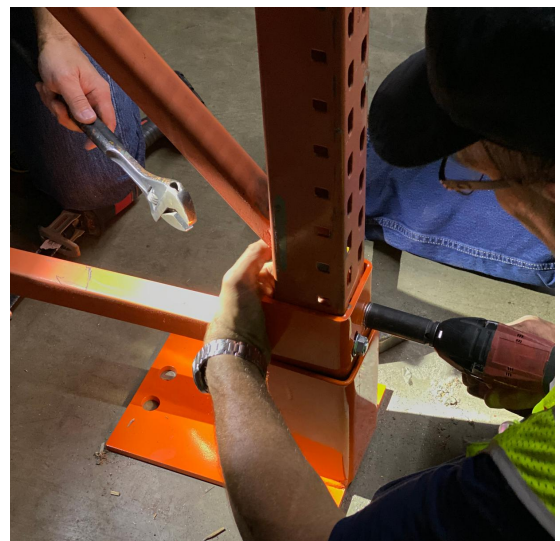
STEP #4 - BOLT & ANCHOR NEW KIT IN PLACE
